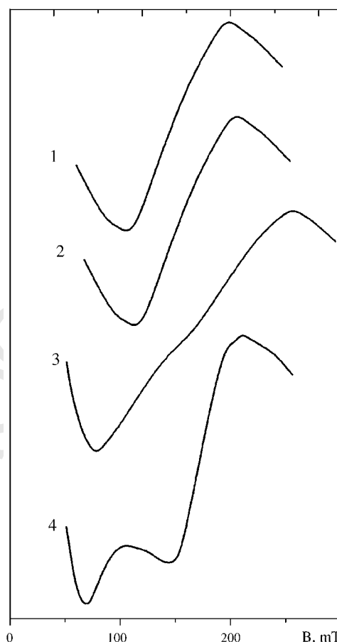
Fig. 3. FMR spectra of \text{La}_{0.7}\text{Sr}_{0.3}\text{Mn}_{1-x}\text{Cu}_x\text{O}_{3\pm\delta} with x = 0 (1); 0.025 (2); 0.05 (3); 0.08 (4). T = 77 K.
