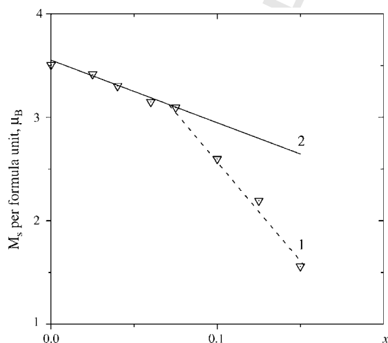
Fig. 2. Measured (1) and calculated (2) saturation magnetization for \text{La}_{0.7}\text{Sr}_{0.3}\text{Mn}_{1-x}\text{Cu}_x\text{O}_{3\pm\delta} at 10 K in the magnetic field of 4000 kA/m.
